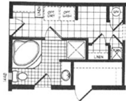
OPTIONAL MASTER BATH WITH REAR ENTRY
